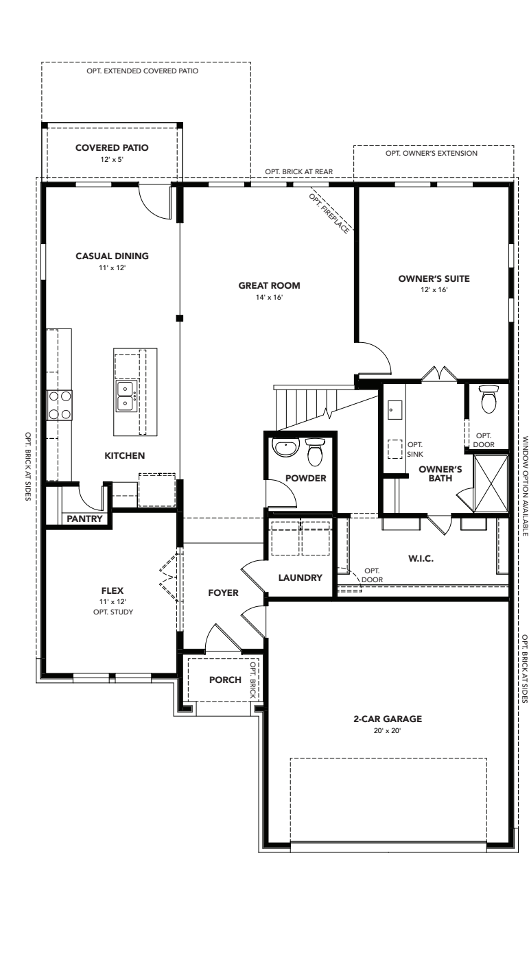
FIRST LEVEL FLOOR PLAN
